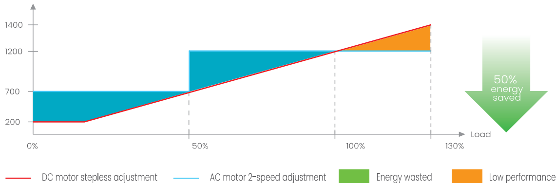
Load-Revolution curve
