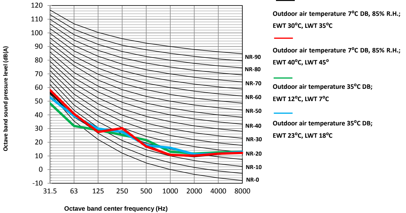
MHA-V8W/D2N8-B + HBT-A100/190CD30GN8-B octave band levels
