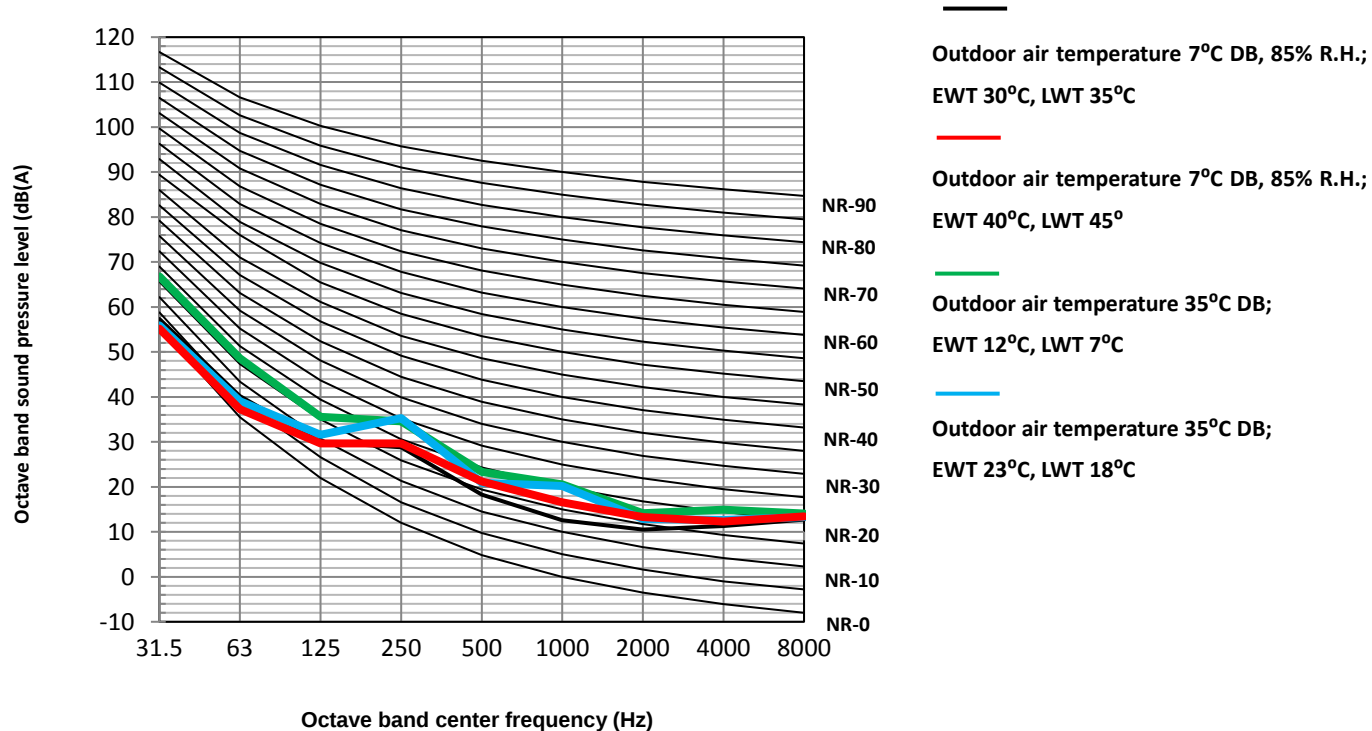
MHA-V16W/D2(R)N8-B + HBT-A160/240CD30GN8-B octave band levels
