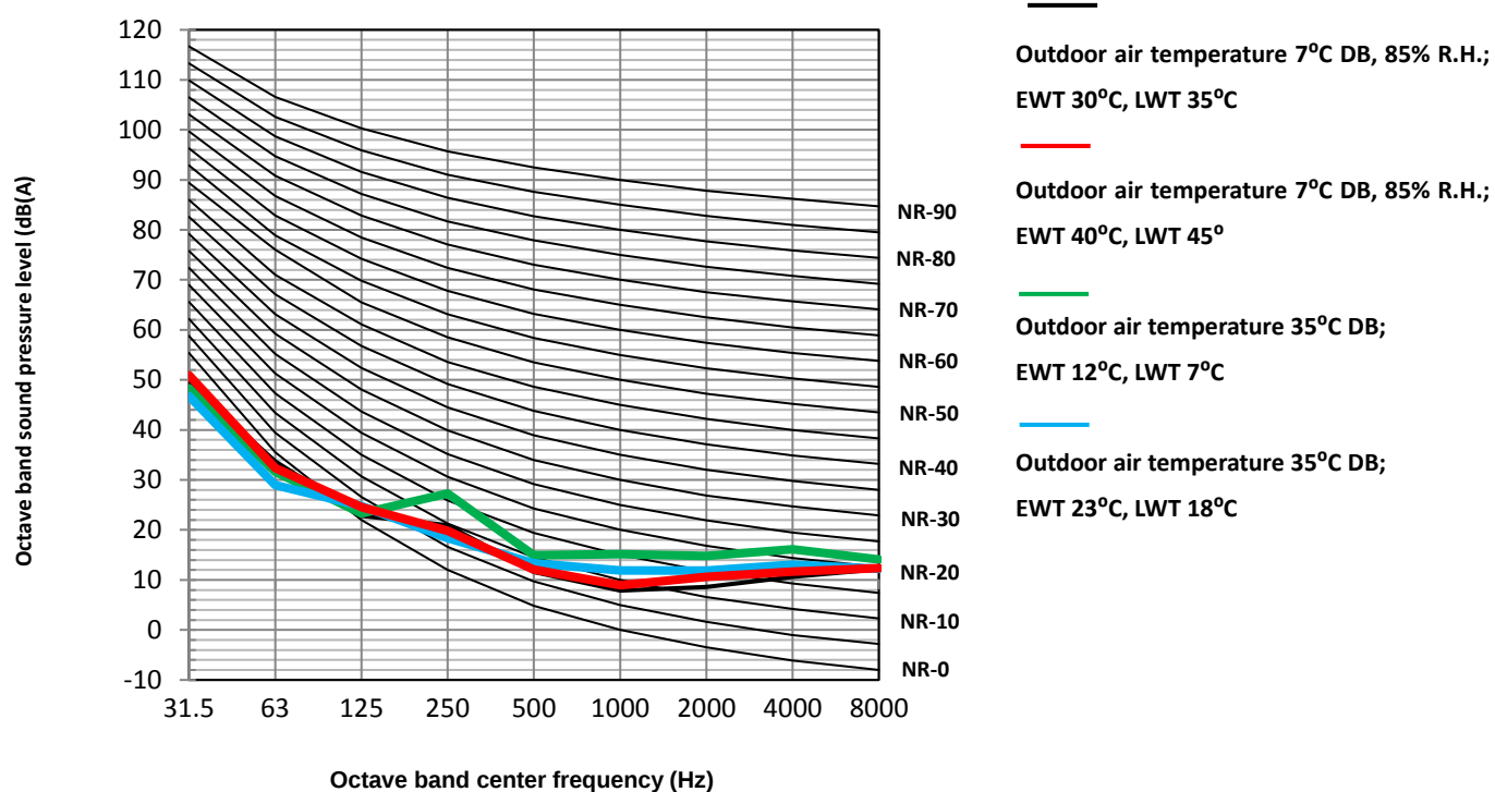
MHA-V4W/D2N8-B + HBT-A100/190CD30GN8-B octave band levels
