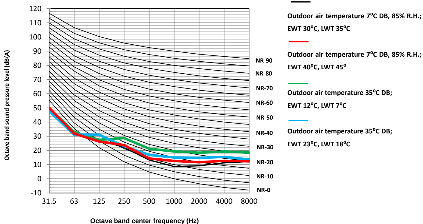
MHA-V6W/D2N8-B + HBT-A100/190CD30GN8-B octave band levels
